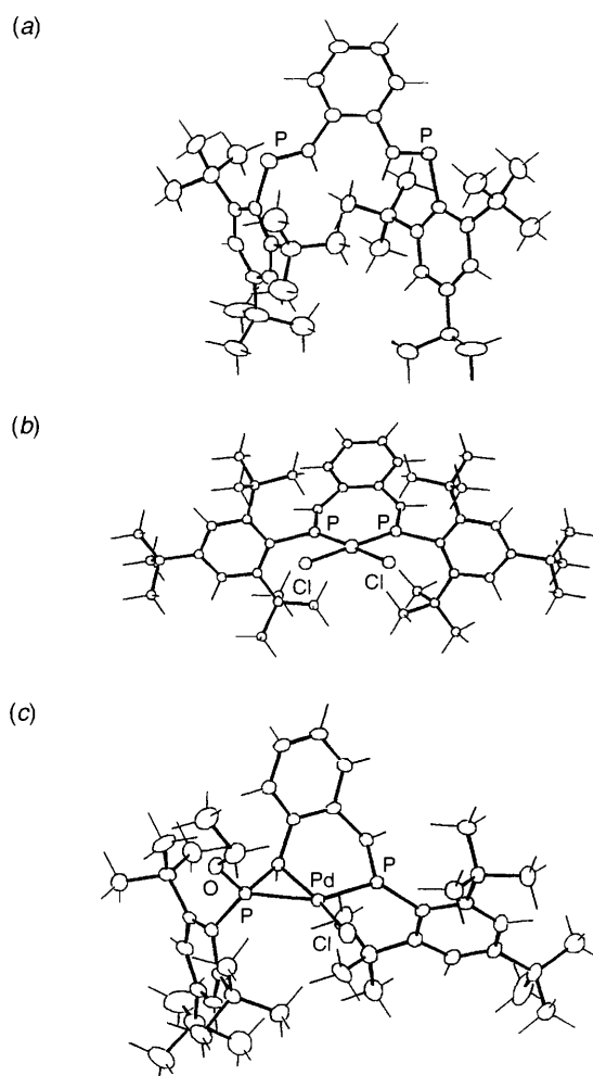
Fig. 1 Perspective views of the crystal structures of L (a), [PdLCl 2 ] (b) and 1 (c). For L and 1 ellipsoids are represented with 50% probability.
